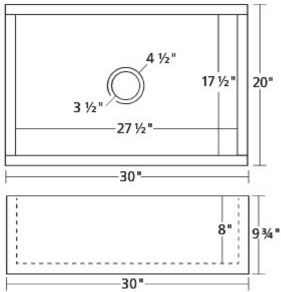
Wright Sink 30" x 20" x 9 3/4" OD
